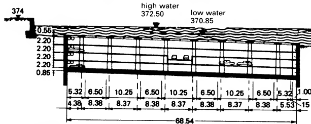
6 Cross-section of 8
